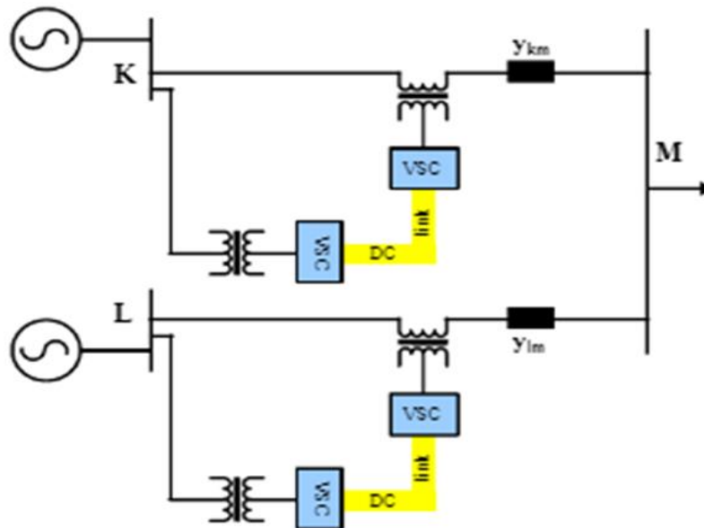
6) IPFC (Interline Power Flow Controller)
