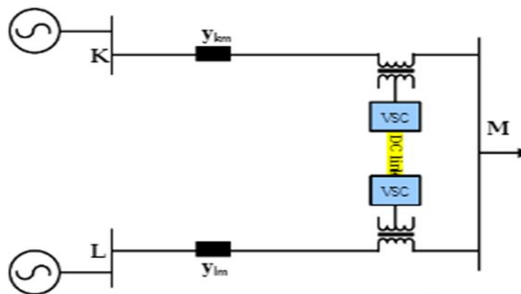
6) IPFC (Interline Power Flow Controller)
