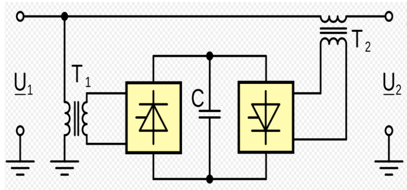
5) UPFC (Unified Power Flow Controller)
